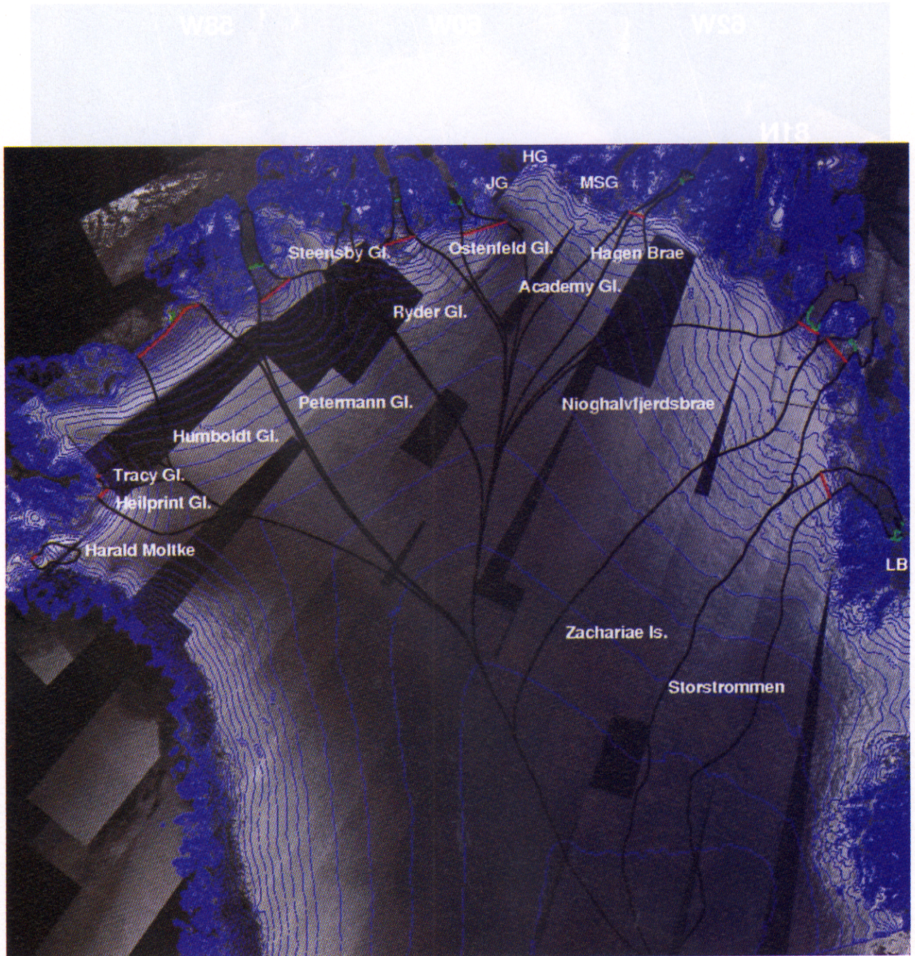
Plate 1. ERS synthetic aperture radar (SAR) mosaic of northern Greenland glaciers on a polar stereographic grid (courtesy National Snow and Ice Data Center, complemented by data from this project). Ice-sounding radar (ISR) lines used to calculate fluxes are shown in red; grounding lines from 1996 are green; drainage basins are black; digital elevation model (DEM) contour lines (every 100 m from 100 m to 2000 m and every 200 m thereafter) are blue. Abbreviations are as follows: JG, Jungersen Gletscher; HG, Henson Gletscher; MSG, Marie Sophie Gletscher; and LB, L. Bistrup Brae. ERS imagery ©ESA 1996.
